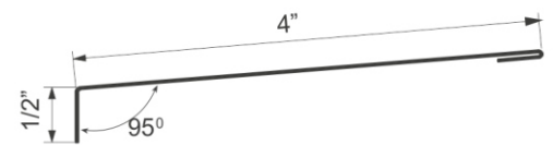
G COUNTER FLASHING
