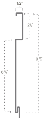
Board & Batten Soffit - Solid
