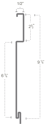
Board & Batten Soffit - Vented
